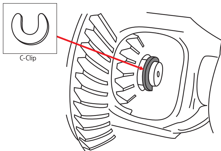
C-Clip style
